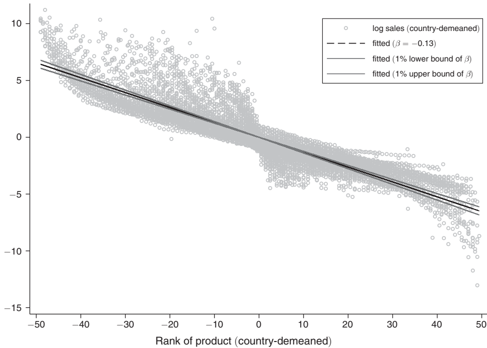
FIGURE C1. REGRESSION YIELDING ESTIMATE OF \vartheta
