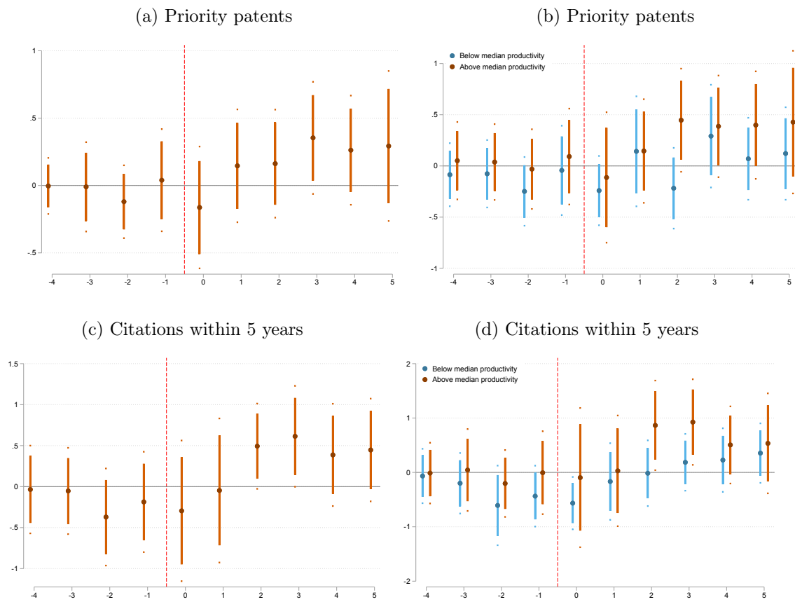
Figure C2: OLS: REMOVING THE MARKETS WHERE A FRENCH FIRM IS A LEADER
