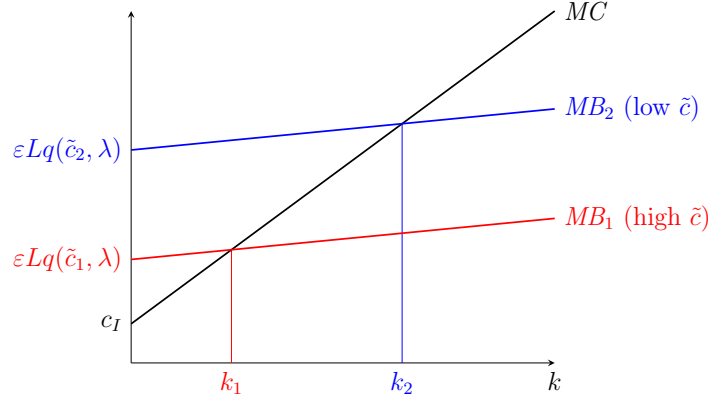
Figure 11: Optimal innovation is higher for more efficient firms
