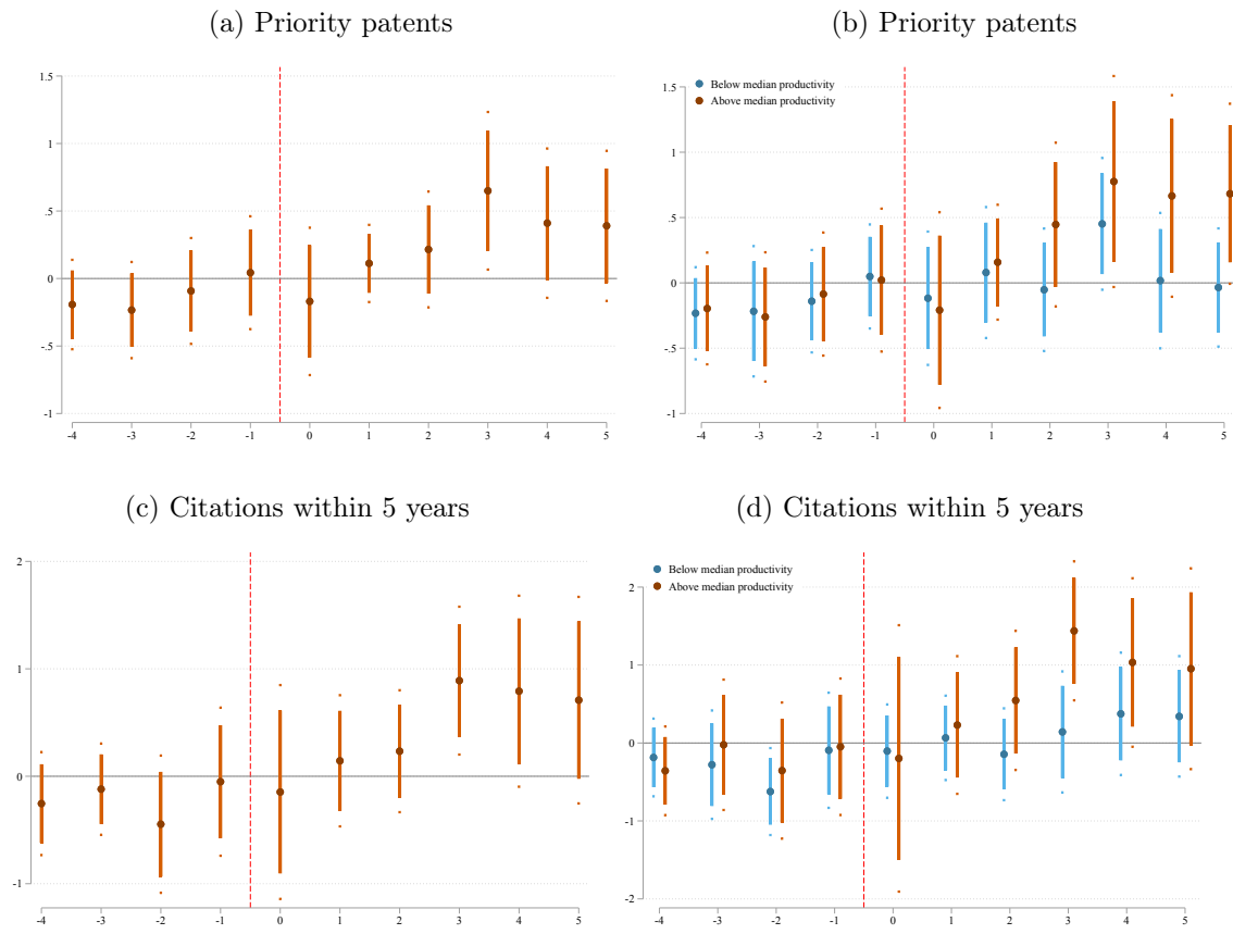
Figure C5: OLS: SAMPLE OF FIRMS WITH t_0 = 1994
